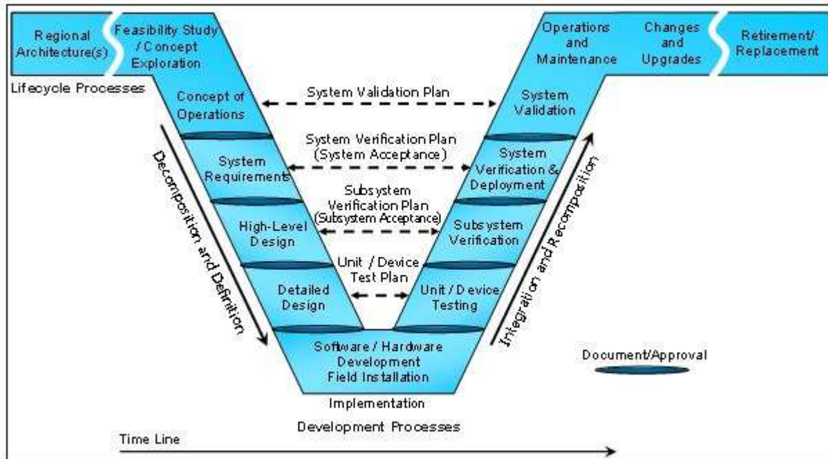
Figure 2. Systems Engineering Decomposition and Integration ‘V’ [2].
