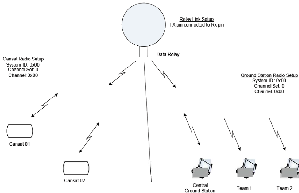
Figure 7: Mission Data Relay Configuration.
