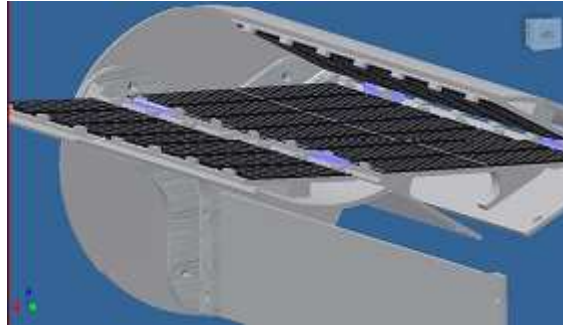
Figure 10: Solar Panel System.
